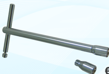
Hose protector installation tool for 3/8 and 7/16 hoses. #SA05 €24 95
