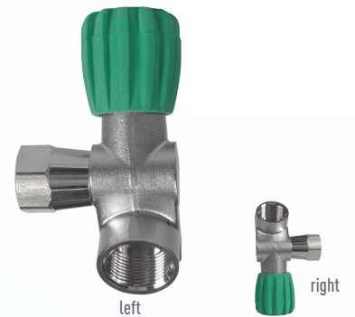
Second outlet M26 232 BAR M25x2 #N10098S left #N10099D right
