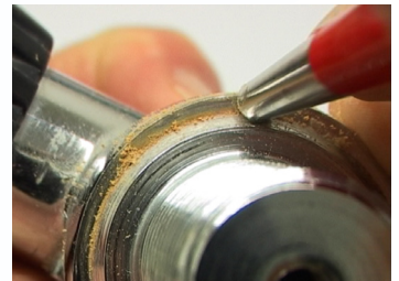
Fiber brush. Glass fiber brush to brush away corrosion. #DTS-FB01
