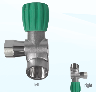
Second outlet M26 300 BAR M25x2 #N10098SD3 left #N10099DD3 right
